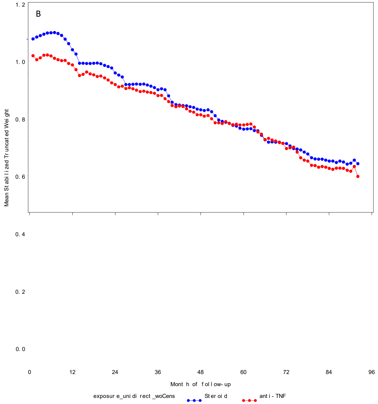
Mean Stabilized Truncated Weights by Month of Follow-up UC patients
