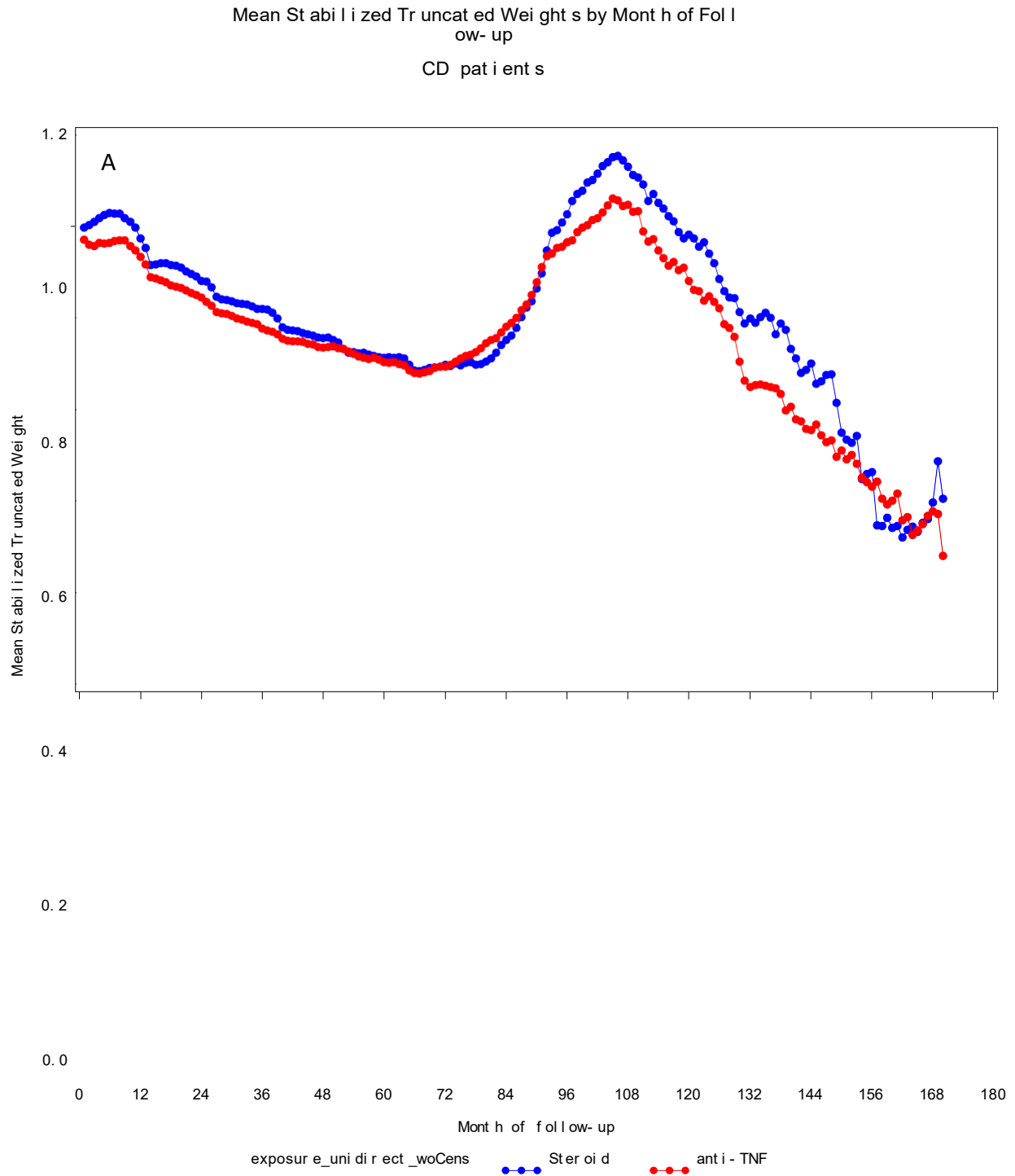
Supplemental Figure 2.1. Mean Stabilized Weights Over Follow-up Time in (A) CD and (B) UC. The increase in the weights that occurs near month 96 in both treatment groups in the CD analysis is attributed to the combination of Medicaid and Medicare data sets allowing for a small subset of the population who had both Medicaid and Medicare benefits and had much longer follow-up time than the other cohort members. Note that the UC analysis included only Medicare beneficiaries.
