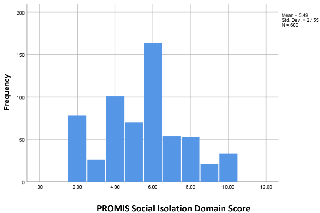
Appendix D, Figure 8: Distribution of PROMIS Social Isolation domain scores among people with osteoarthritis of the knee in the cross-sectional sample
