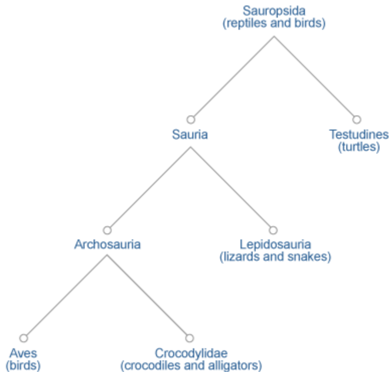
Figure 1. A phylogenetic classification scheme. If two organisms (A and B) are listed more closely together in the taxonomy than either is to organism C, the assertion is that C diverged from the lineage leading to A+B earlier in evolutionary history, and that A and B share a common ancestor that is not in the direct line of evolutionary descent to species C. For example, the current consensus is that the closest living relatives of the birds are the crocodiles; therefore, our classification does not include the familiar taxon Reptilia (turtles, lizards and snakes, and crocodiles), which excludes the birds, and would break the phylogenetic principle outlined above.
