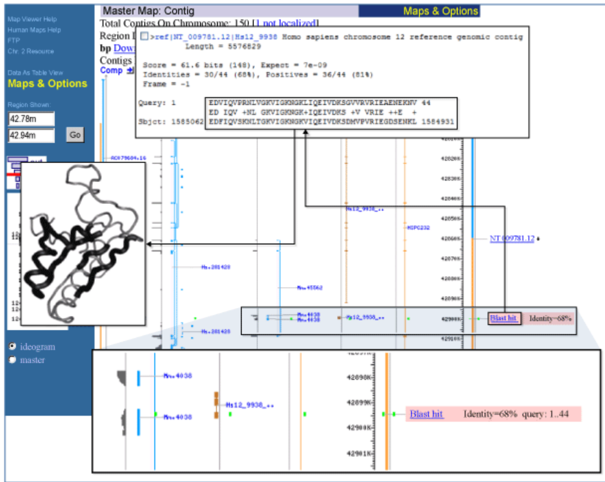
Figure 8. BLAST hits.
